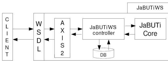
Fig. 3. Architecture of the JaBUTiWS.
