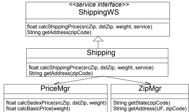
Fig. 6. Class Diagram of ShippingWS.
